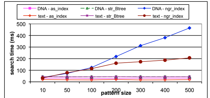
Figure 6: Search result on 100MB files, for varying pattern size
