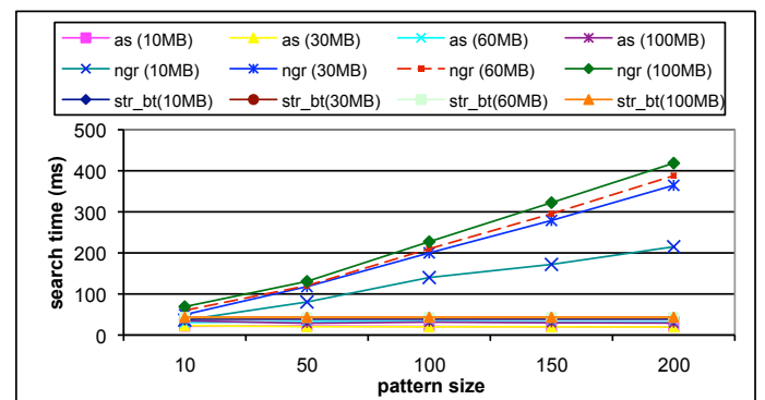
Figure 7: Search result, for varying pattern and file size
