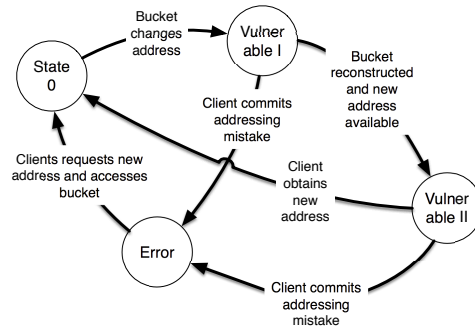
Fig. 15 Markov state model for determining addressing mistakes based on a wandering bucket.
