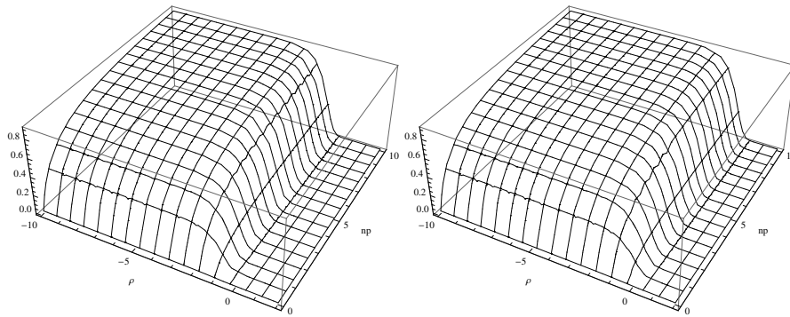
Fig. 16 Probability for not committing an address error for bucket access rate \lambda = 10^9 , -10 \leq \rho \leq 2 per second, T_r = 10\text{sec} (left) and T_r = 2\text{sec} (right), and values of np between 1/100 and 10 .
