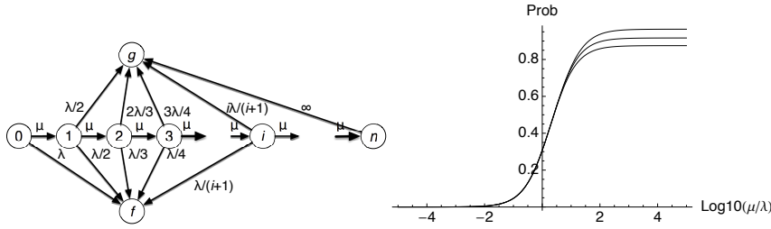
Fig. 13 Left: Markov model for the evaluation of gossiping. Right: Probability of not committing an address error (with 7, 11, and 27 buckets from bottom to top).
