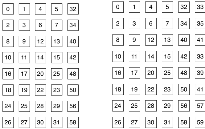
Fig. 12 Left: Bucket allocation where category A has file state j_A = 2 and s_A = 1 , category B has file state j_B = 3 and s_B = 0 and mixing vector (011010) . Right: Bucket allocation after changing the category A file state to j_A = 2 and s_A = 2 .
