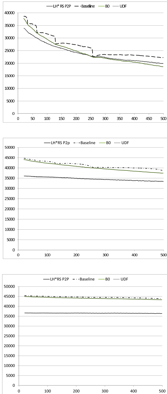
Fig. 14 Non-compulsory single forwarding messages in the low, moderate, and fast growth scenario depending on the starting size (in buckets) of the LH* file.
